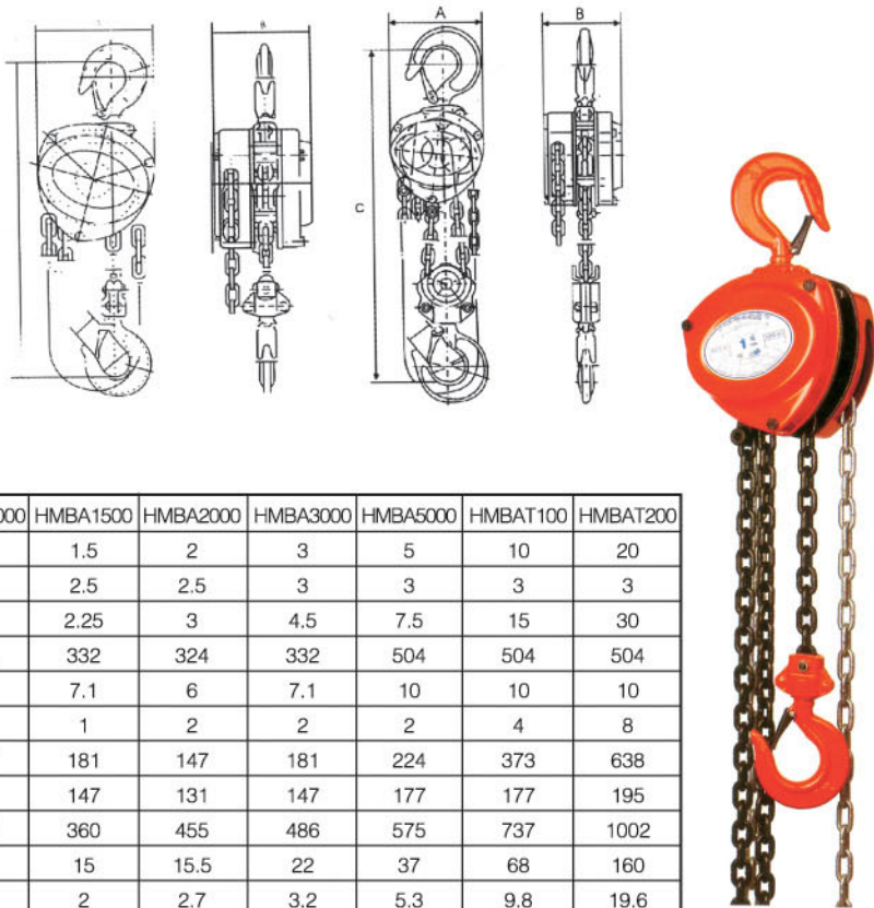
HMBA Type Chain Blocks
