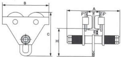
Push Trolley HPTC Type
