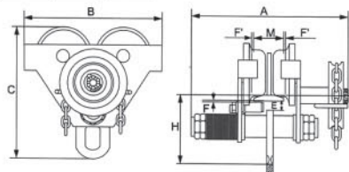
Gear Trolley HGTC Type
