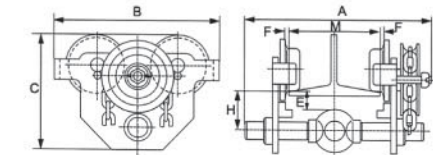
Gear Trolley HGTF Type
