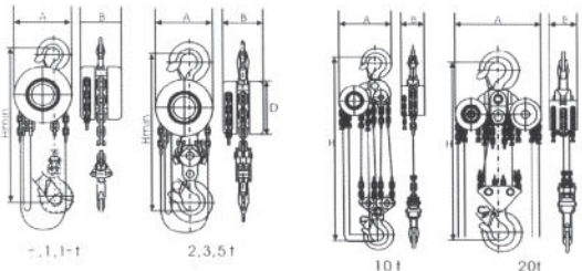
HMBE Type Chain Blocks
