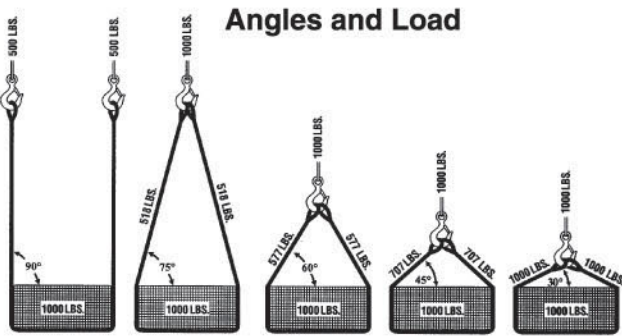
Sling Angles
