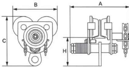
Gear Trolley HGTB Type
