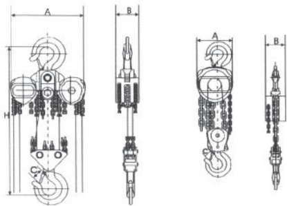
HMBJ Type Chain Blocks
