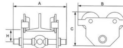
Push Trolley HPTF Type
